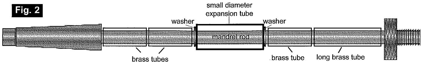
Reed Assembly
