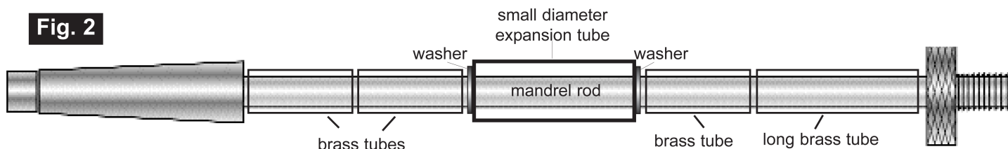
Reed Assembly
